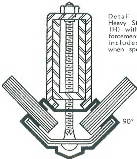
CORNER BAR No. 921
